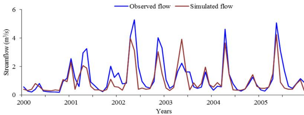
Figure-4. Monthly streamflow calibration results for RGS 4CB05.
