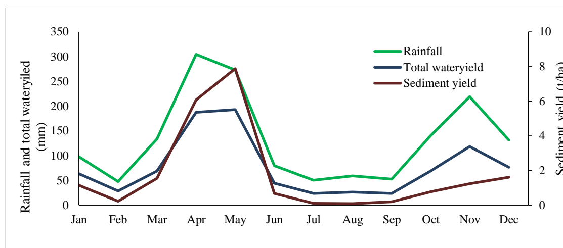
Figure-7. Average monthly sediment and water yield in Thika river catchment.
