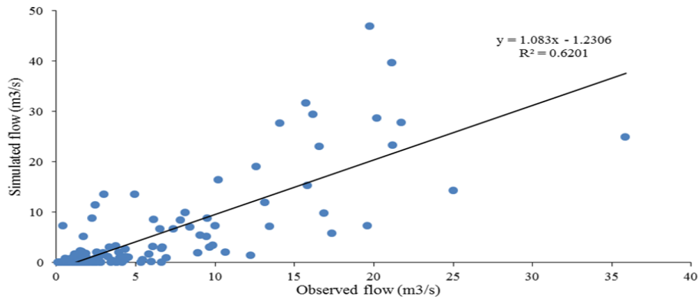
Figure-7. Plot of observed and simulated streamflow at gauging station 4CB04.
