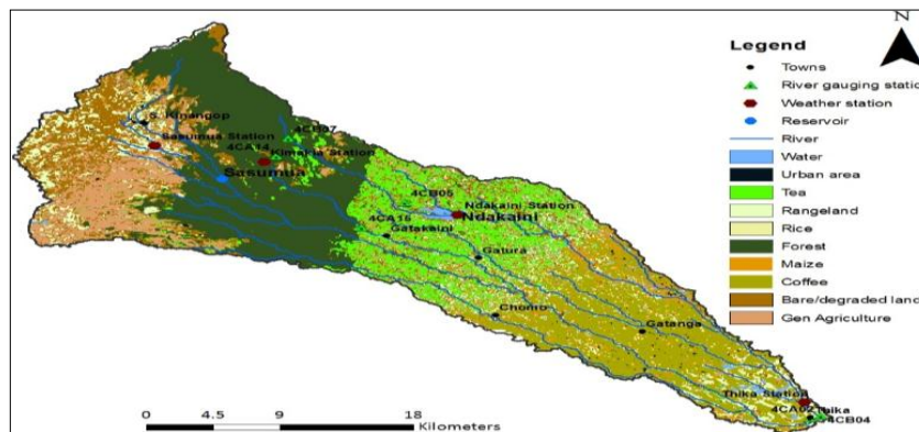
Fig-2. Land-use/cover in Thika river catchment.
